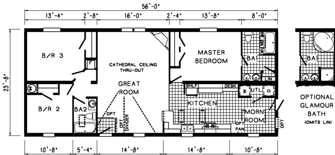
2A103-A 2456 Approx. 1325 Sq. Ft.
