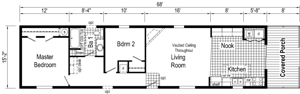
1A111-A 1668 Approx. 910 Sq. Ft.
