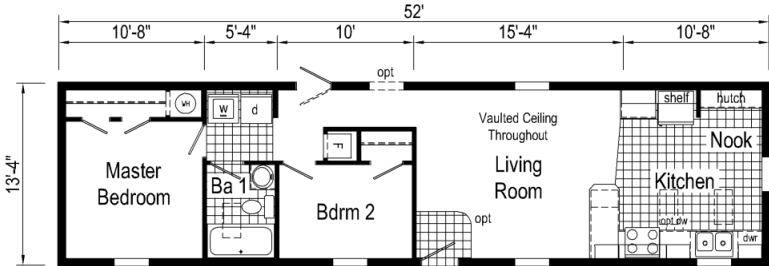
4A127-A 1452 Approx . 693 Sq. Ft.
